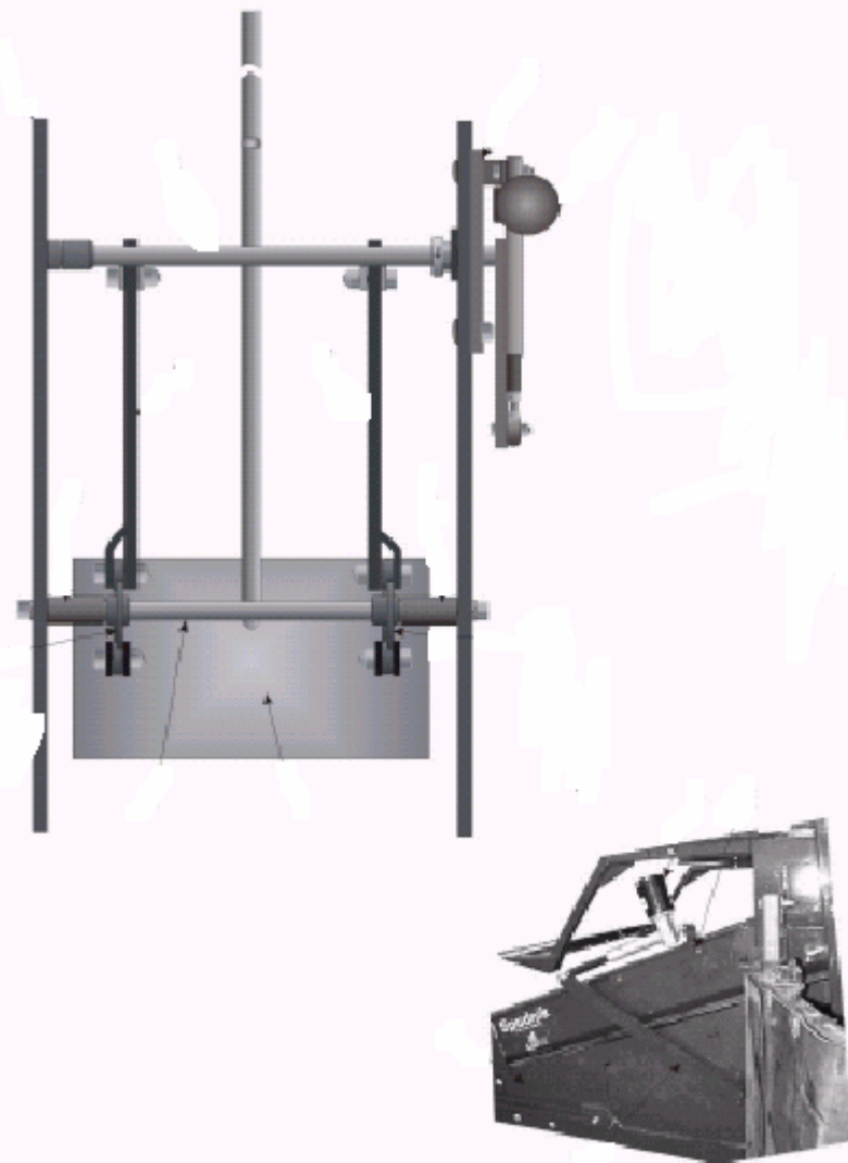
NOSE SKID PAN ACTUATOR ADJUST ASSEMBLY (OPTION)
