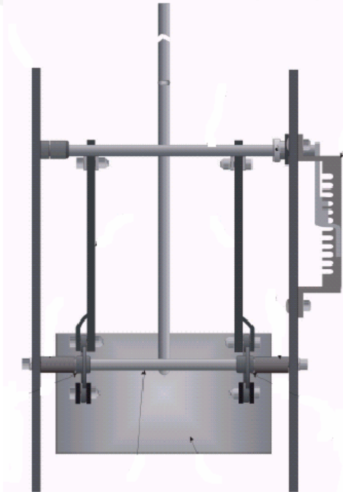
NOSE SKID PAN HAND ADJUST ASSEMBLY (STANDARD)
